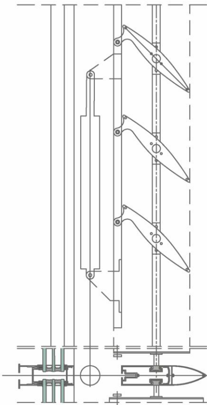
CROSS SECTION OF BRISE SOLEIL YAWAL SUN PROTECTION - MOBILE VERSION
