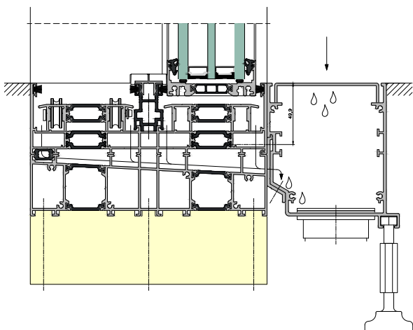
LINEAR DRAINAGE WITHIN THE MOREVIEW SYSTEM
