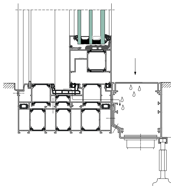
LINEAR DRAINAGE WITHIN THE DP 180 SYSTEM
