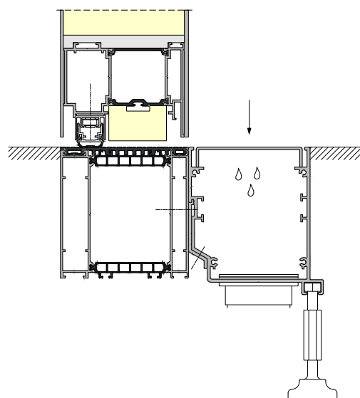
LINEAR DRAINAGE WITHIN THE TM 102HI SYSTEM
