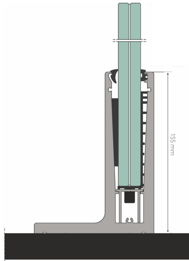
CROSS SECTION OF BA 50 BALUSTRADE SYSTEM
